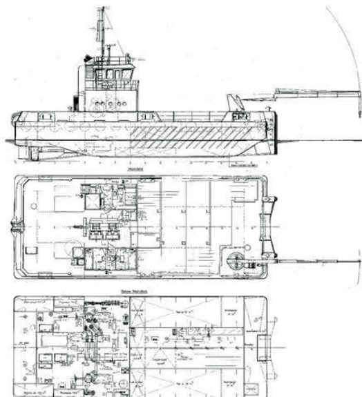
Port Servicer's general arrangement
