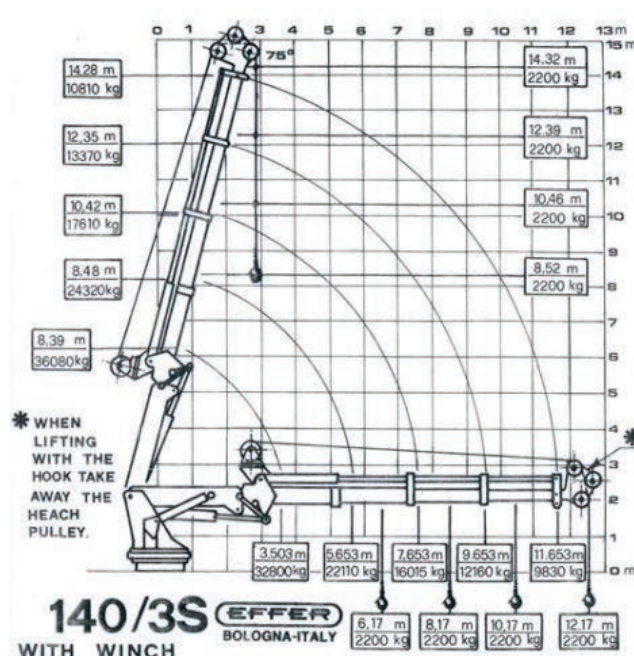
Port Servicer's crane load chart
